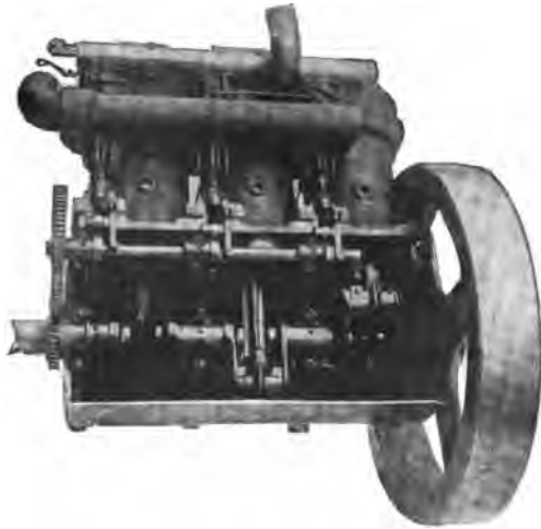
FIG 307.—The Duryea Three-Cylinder Gasoline Vehicle Engine, with half the crank case sheathing removed, showing cranks, crank shaft, cam shaft, and working parts. The three cylinders have common supply and exhaust tubes; the charge is controlled by a single throttling link, shown at the top, and the igniting circuit has three bridges for the three cylinders
